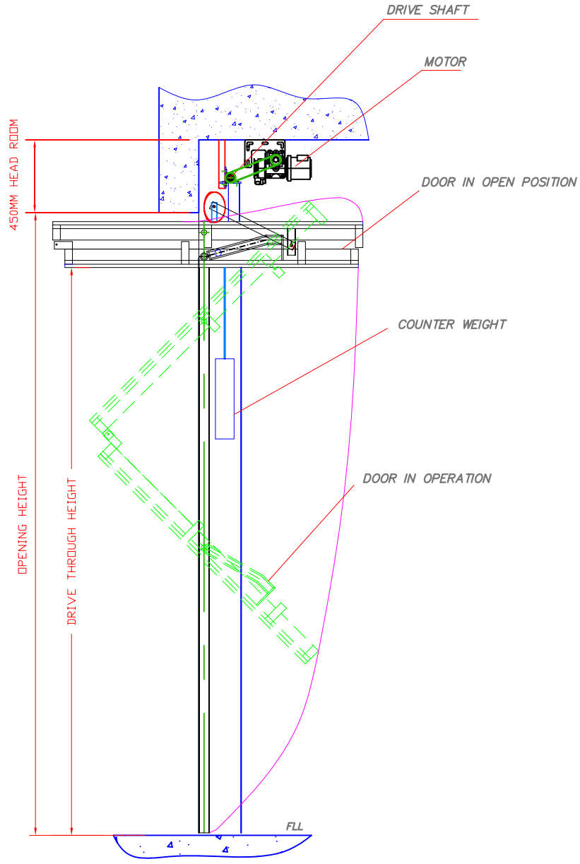
SIDE VIEW
