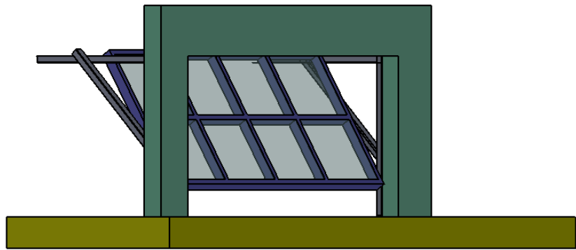
OUTSIDE VIEW - DOOR IN OPERATION
